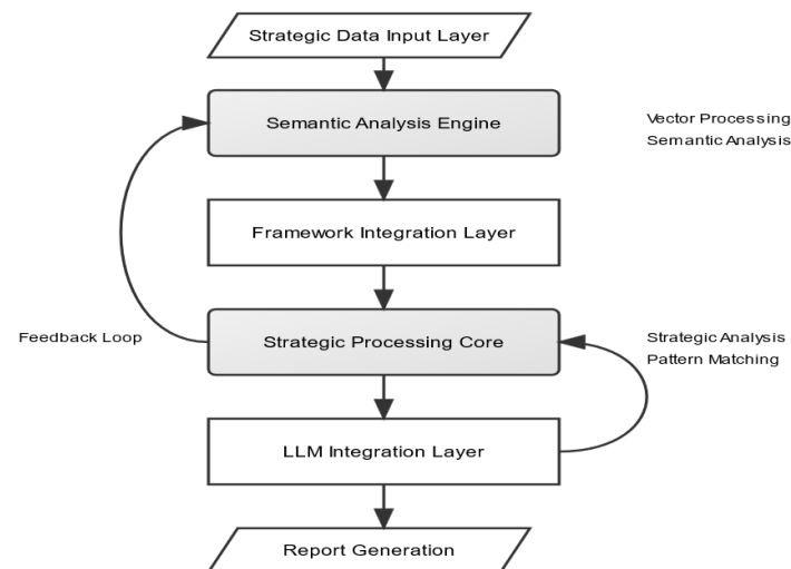
Figure 1. Computational architecture overview.
